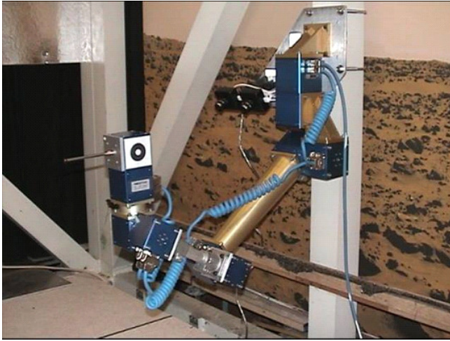
Figure 14. modular arm and camera system used for experiments
