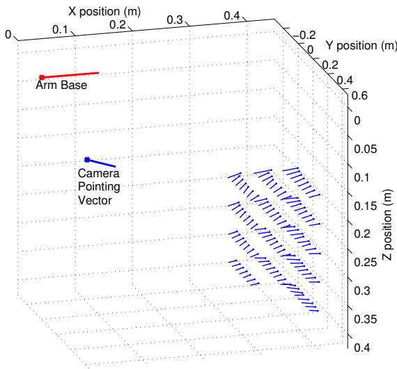
Figure 15. correction vector field for experimental system, plotted in world coordinates with arm base and camera location
