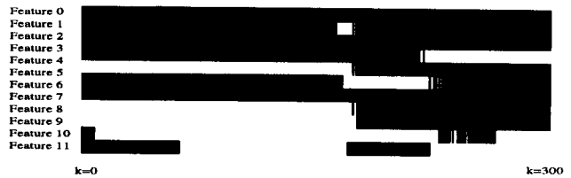
Figure 4: Feature Visibility
