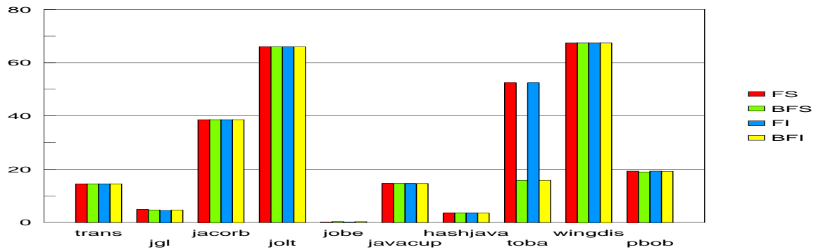
Figure 9: Percentage of user local object space allocated on the stack.
